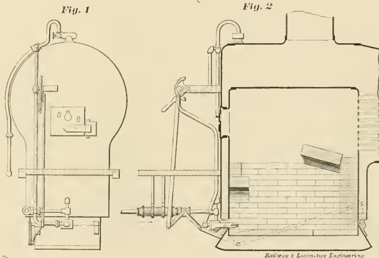
REGULATOR FOR OIL-BURNING LOCOMOTIVES.
